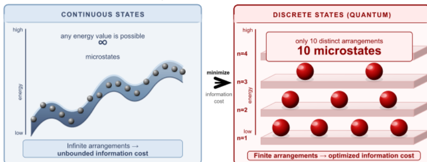
Figure 9 - 1 Continuous systems carry an unbounded information cost; discrete systems minimize it. If physical reality optimizes information storage, discreteness is the predicted outcome, precisely what quantum mechanics shows.
